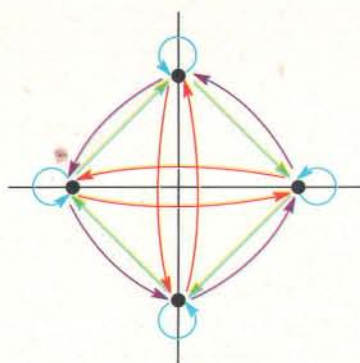
Figure 2: Four-state differential phase-shift keying. This phase-amplitude diagram shows a set of states and transitions for a four-state DPSK modulation scheme.
